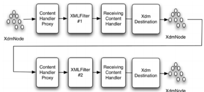
Figure 1: Adjacent java filters linked via Xdm trees
